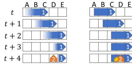
Figure 1: A k R-MAPF plan with no collisions (left) and an MTPF plan with a collision at D at timestep t + 4 (right). In both figures, agent 1 moves from left to right across the map. Its location is C at timestep t , and it waits for two timesteps once at E. Meanwhile, agent 2 enters D at timestep t + 4. The number of vertices occupied by an agent in k R-MAPF shrinks when the agent is waiting. However, an agent in MTPF always occupies multiple vertices at each timestep.
