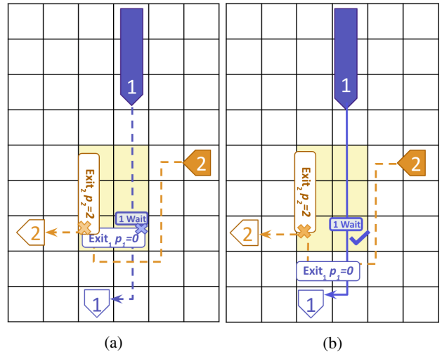
Figure 3: (a) Rectangle conflict between two agents. We place barrier constraints that forbid each agent from exiting the rectangle area at their currently optimal time. Each barrier is extended in the temporal dimension by a number of timesteps equal to the body length of the other agent. The dashed lines indicate a valid MTPF plan (where the blue agent waits for one timestep at the blue-crossed vertex) that violates both barrier constraints at the respective crossed vertices. (b) The blue barrier is pushed away by one step from the yellow rectangle area. Now, the blue path does not violate the blue barrier constraint. Thus, the plan satisfies the disjunction of the two barrier constraints.
